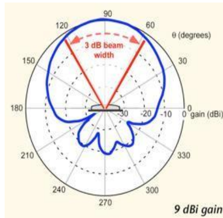
Figure 1.4: A polar diagram showing beamwidth.
